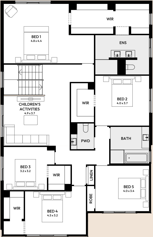
FIRST FLOOR
