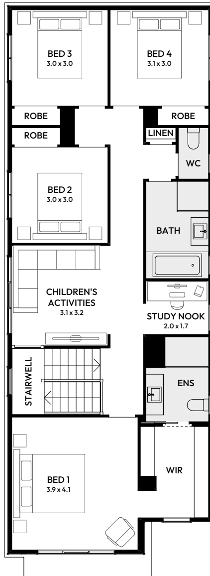
FIRST FLOOR
